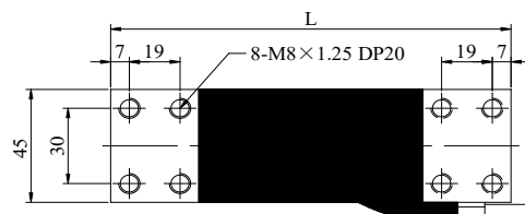
俯視(Top View)
