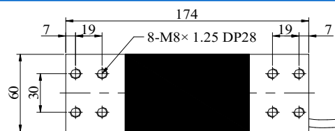
俯視 (Top View)
